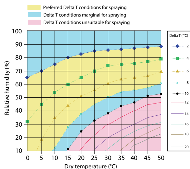
Figure 14. Delta T chart indicating appropriate conditions for spraying.
