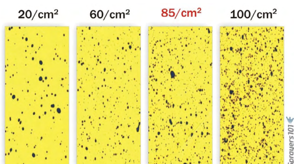
Figure 15. 85 droplets per square centimetre provides the appropriate coverage. Photo: Jason Deveau, Sprayers 101.
