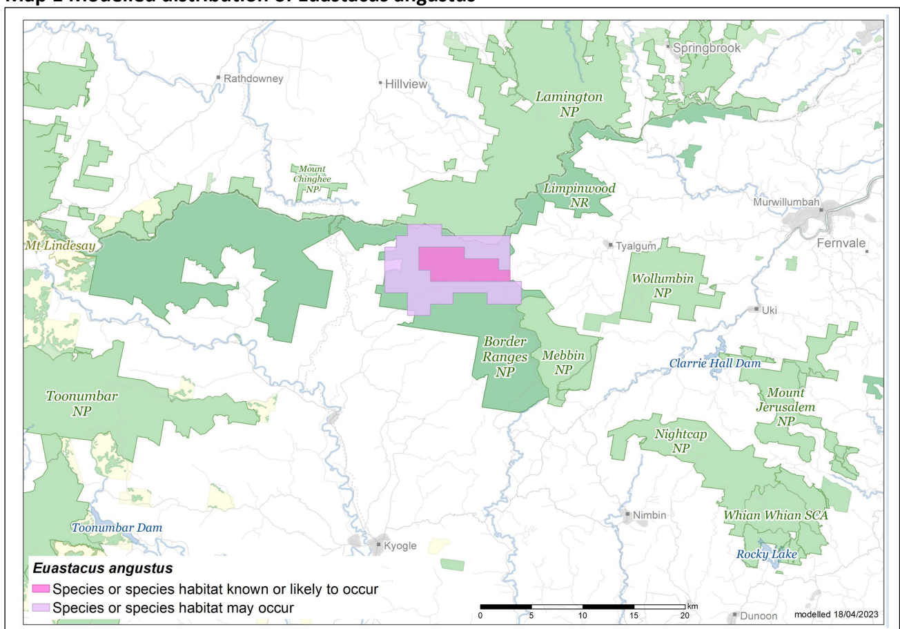
Map 1 Modelled distribution of Euastacus angustus
