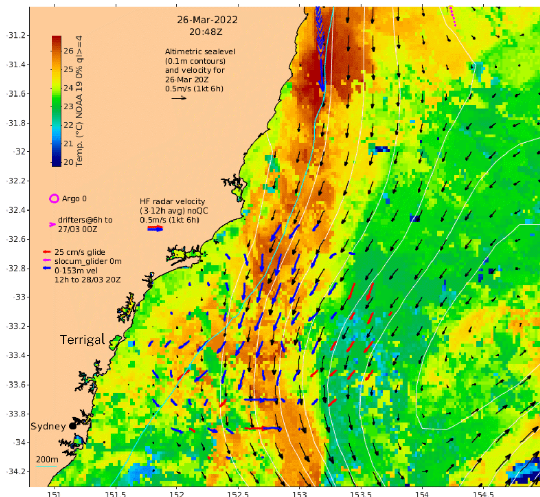
Figure 22 Tasman Sea currents and sea temperatures for 30 March 2022 Source: IMOS 2022
