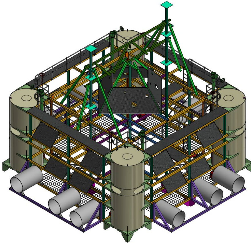
Figure 9 Final design of Terrigal offshore artificial reef steel structures
