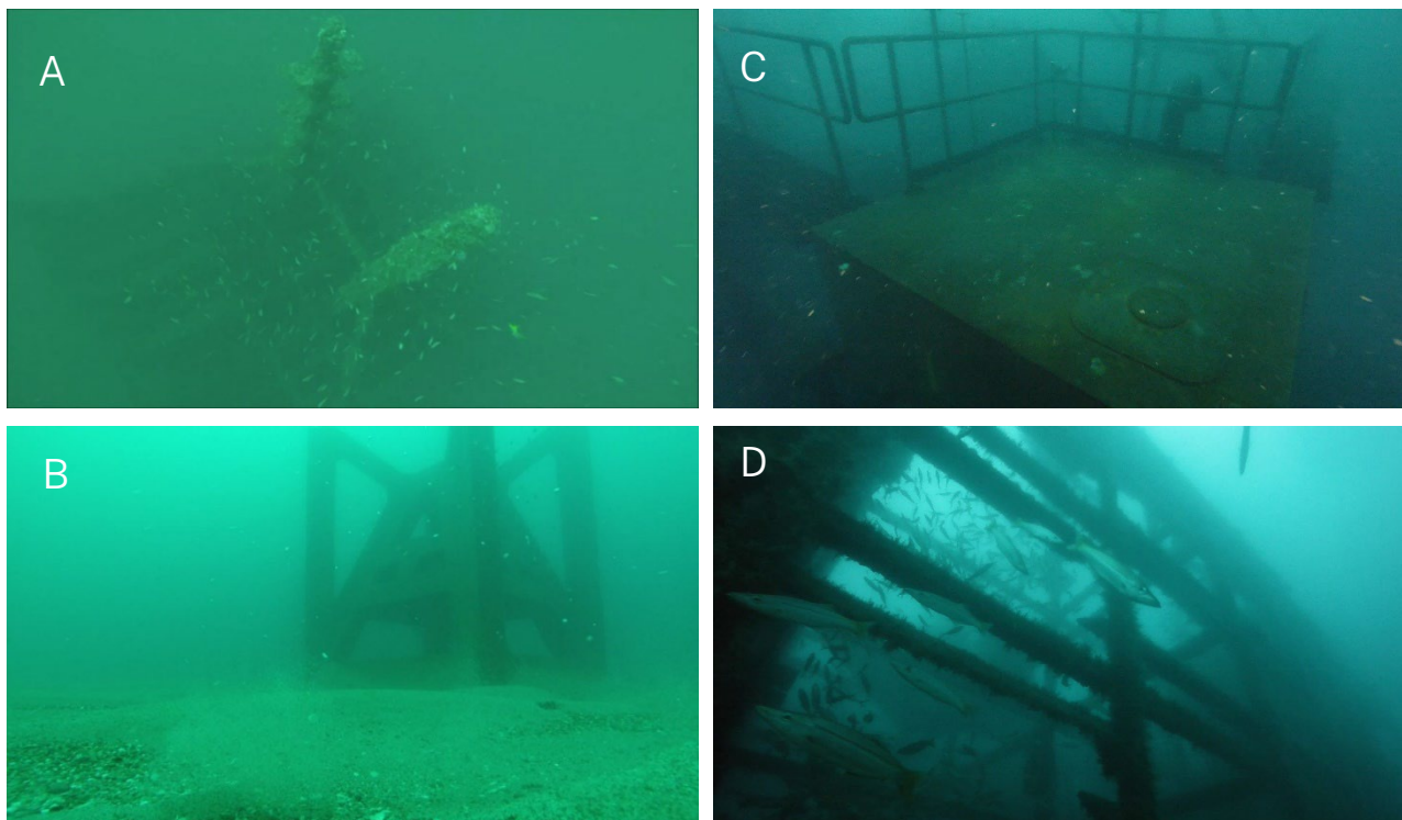
Figure 23 Inspections of A) Sydney (7 May 2015), B) Shoalhaven (18 May 2015) and C, D), Eurobodalla (July 2022, Credit: SMC Marine) offshore artificial reefs following intense east coast low events that produced waves over 15 m (Hmax).
