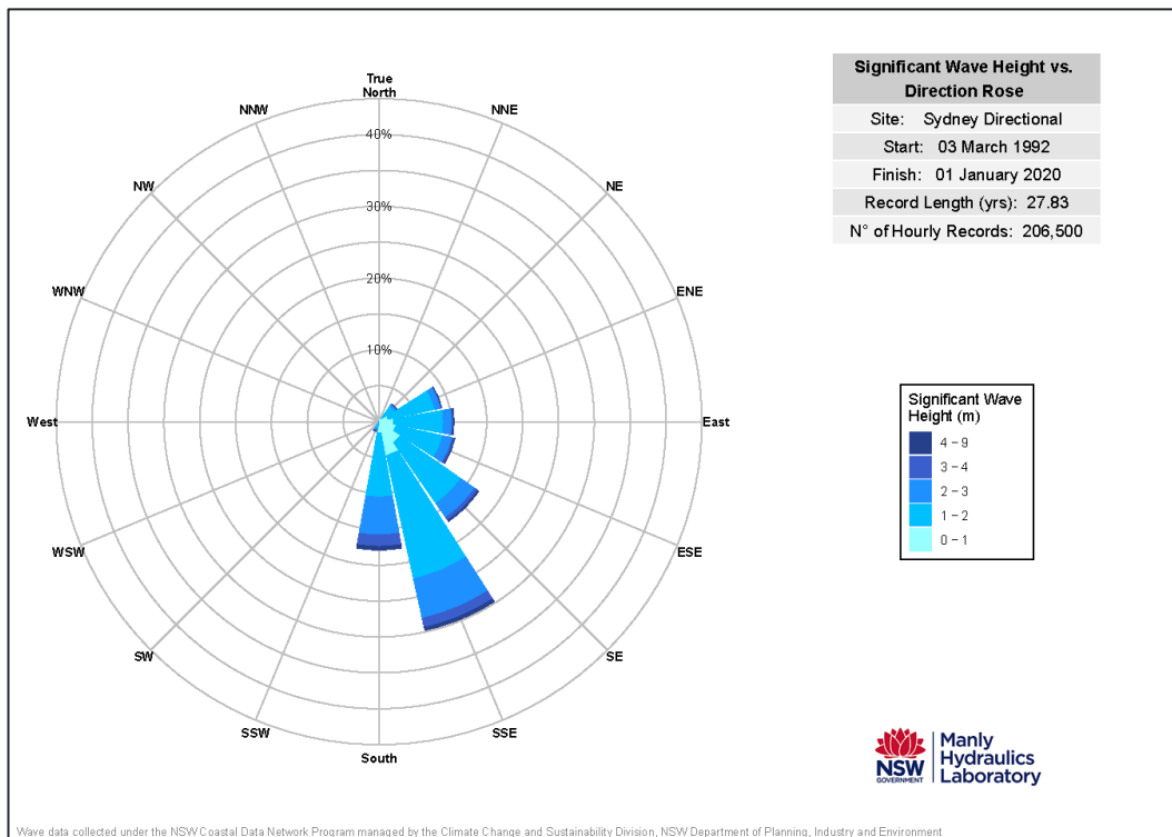
Figure 20 Wave rose of Sydney offshore wave dataset
