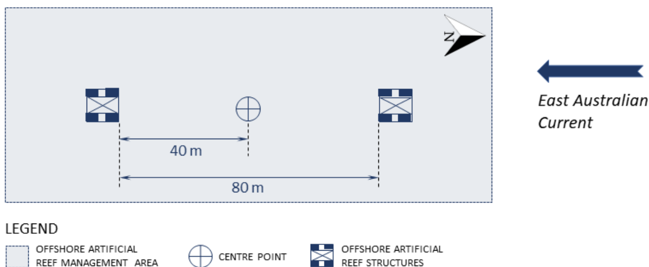
Figure 13 Terrigal offshore artificial reef structures arrangement
