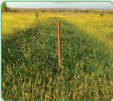
Rundown affected buffel pasture response to nitrogen application (dark green middle strip). SRB
