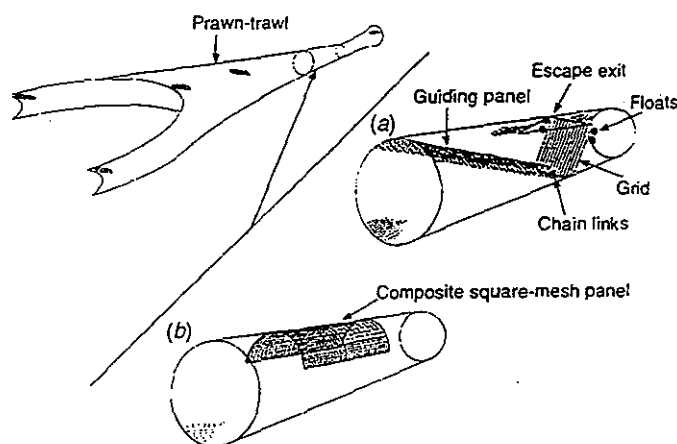
Fig. 1. Diagrammatic representation of a prawn-trawl and location of (a) the Nordmøre-grid and (b) the composite square-mesh panel.
