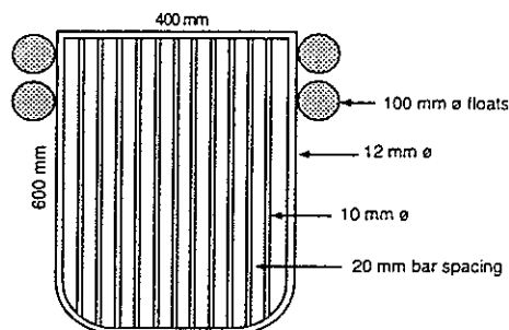
Fig. 3. Aluminium grid used in the standard and modified Nordmøre grids.
