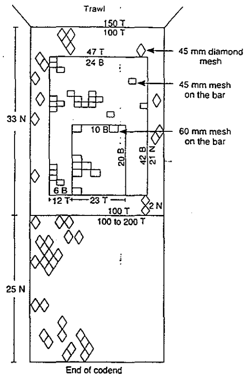
Fig. 6. Diagrammatic representation of assembled composite square-mesh panel.
