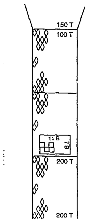
Figure 3. Diagrammatic representation of a modified codend incorporating a square mesh panel as tested in the Clarence River oceanic prawn trawl fishery. T = transversals, B = bars (from Broadhurst et al. 1996b).
