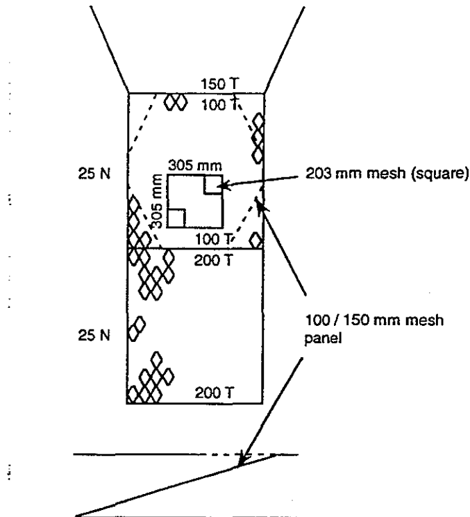
Fig. 4. Diagrammatic representation of the 100 mm and 150 mm SPCs trialed in the Botany Bay Experiment and Clarence River Experiment 3.
