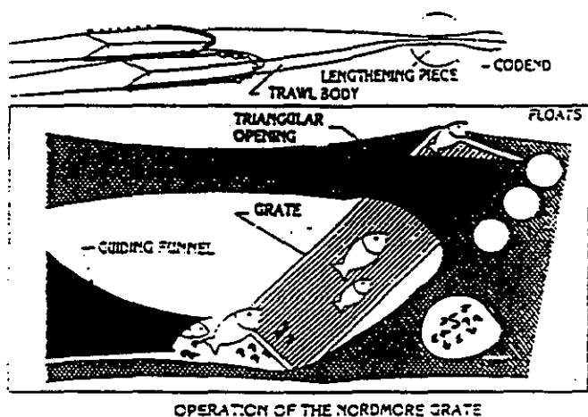
Fig. 7. Schematic representation of the operation of the Nordmore Grid.
