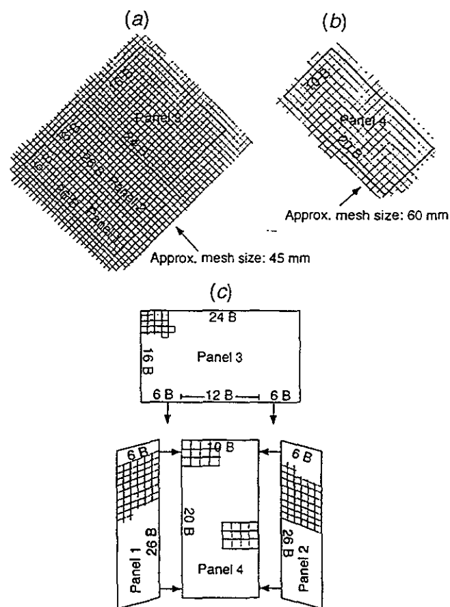
Fig. 5. Composite square-mesh panel: diagrammatic representation of netting required for (a) Panels 1, 2, 3 and (b) Panel 4; (c) assembly.
