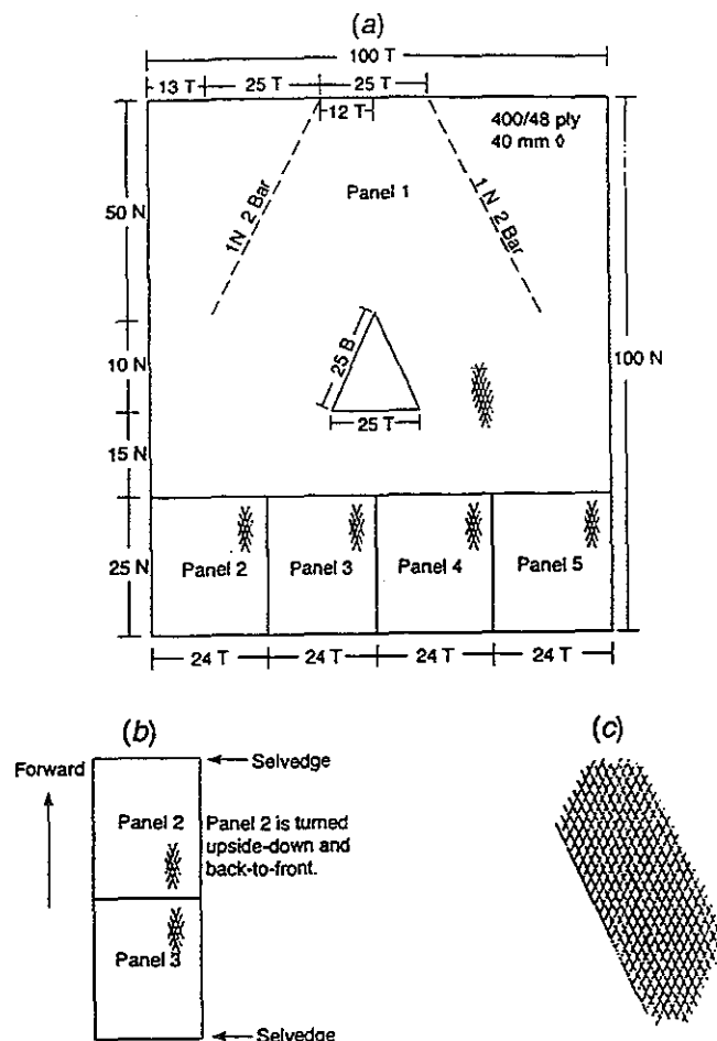
Fig. 3. Nordmøre-grid: diagrammatic representation of (a) netting panels, (b) guiding-panel assembly and (c) 1-normal 2-bar taper.
