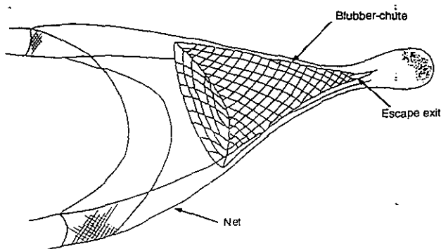
Fig. 2. Diagrammatic representation of the commercially used blubber-chute and trawl.
