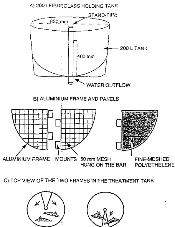
Fig. 1. Diagrammatic representation of: (A) the 200 l fiberglass tanks, (B) the aluminium frames and panels used in the experiments and (C) the frames being rotated together in the treatment tanks (top view).
