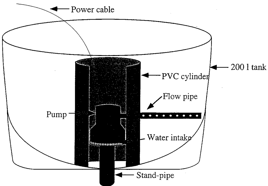
B) 200 l tank with pump assembly attached
