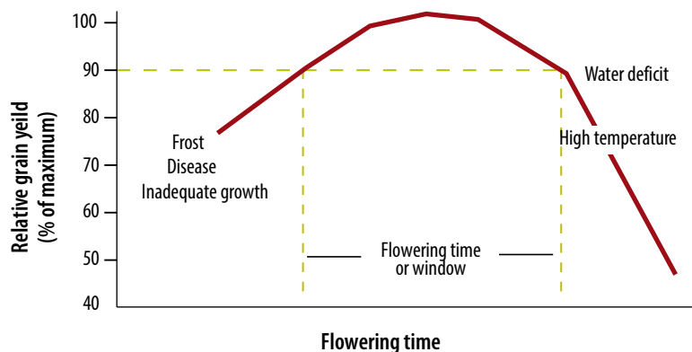
Figure 3-12: The flowering window. The optimum flowering time depends on location and the acceptable frost risk. Source: Based on W Anderson & J Garlinge, 2000.
