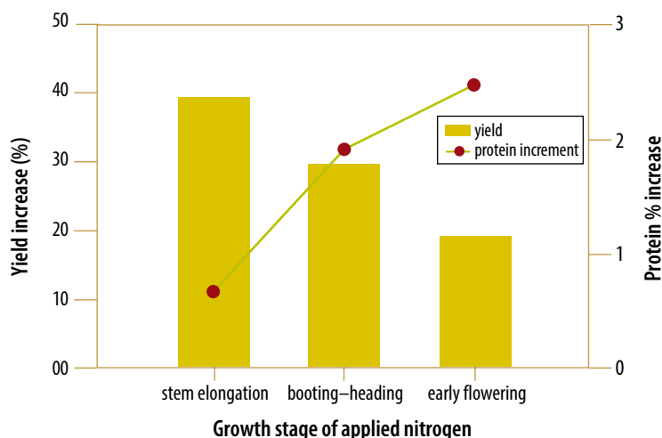
Figure 3–16: Effect of applying 100 kg N/ha (as urea) at various growth stages on yield and protein of commercial wheat crops in 1993. Source: Based on B Manning et al., 1998.
