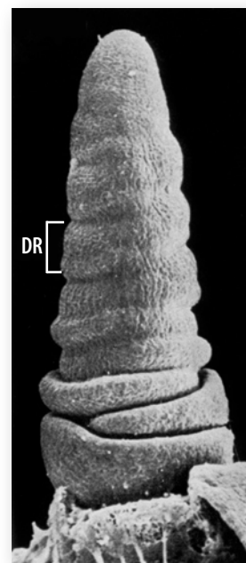
Figure 3–2: The changes in the elongating apex as the double ridges (DR) begin to form. Source: CSIRO.
